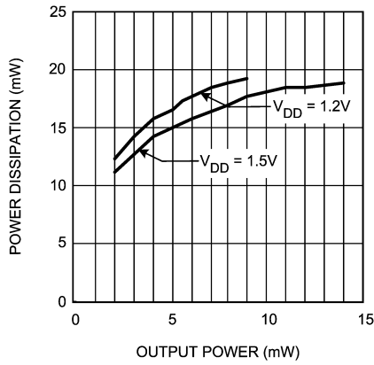
Power Dissipation vs Output Power f = 1kHz, THD+N < 1%, A_V = -1 Single Ended Output, Both Channels
